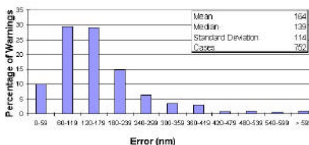
Figure 5-2e Frequency distribution of 48-hour track errors for western North Pacific Ocean tropical cyclones in 1997. The largest error, 891 nm, occurred on Tropical Storm Levi (05W).
